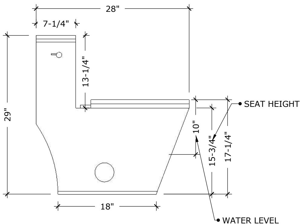
SIDE ELEVATION
