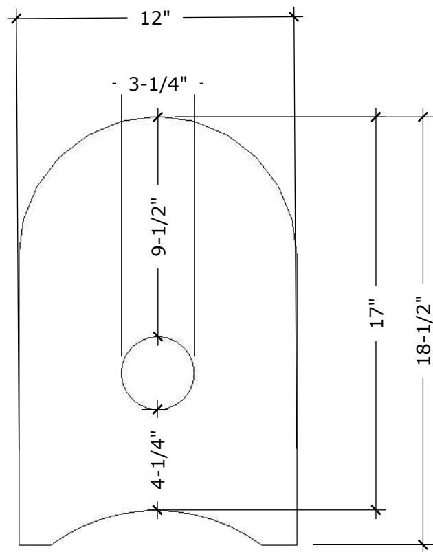
BOTTOM VIEW
