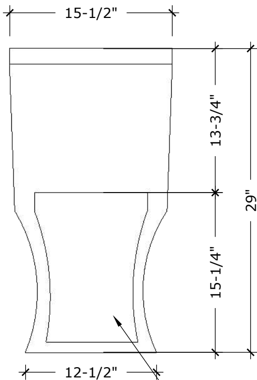
BACK VIEW
