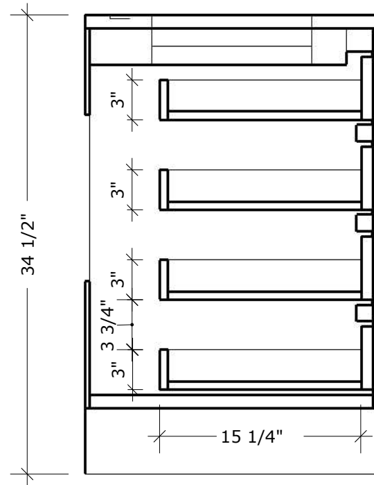
SECTION CUT
